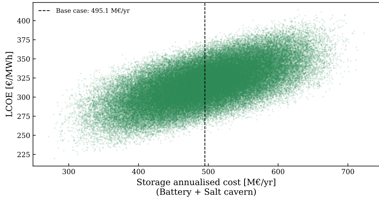
LCOE vs Storage annualised cost
